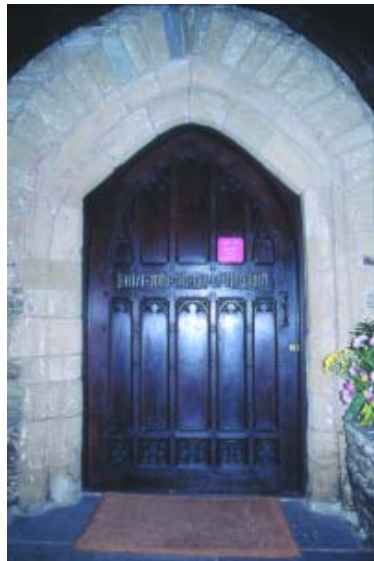
10. An arch built of Quaternary sandrock in St Carantoc's church at Crantock. A tower built of this sandrock in the 14th century fell down shortly after it was built, suggesting that there are structural limitations with this type of stone. (c. Colin Bristow)
